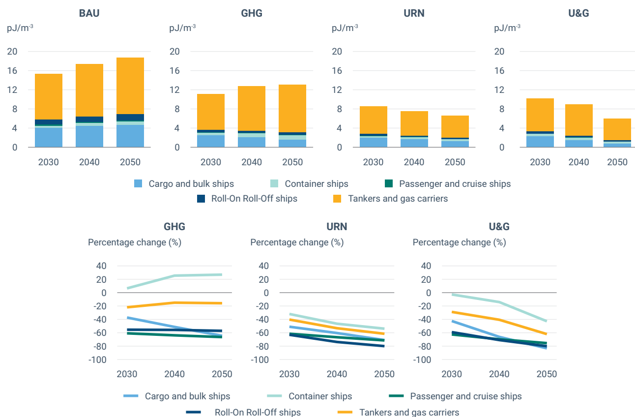
Figure 2.36 URN forecast scenarios Sound Energy Density (top) and Mitigation Performance (bottom) for the Mediterranean Sea
