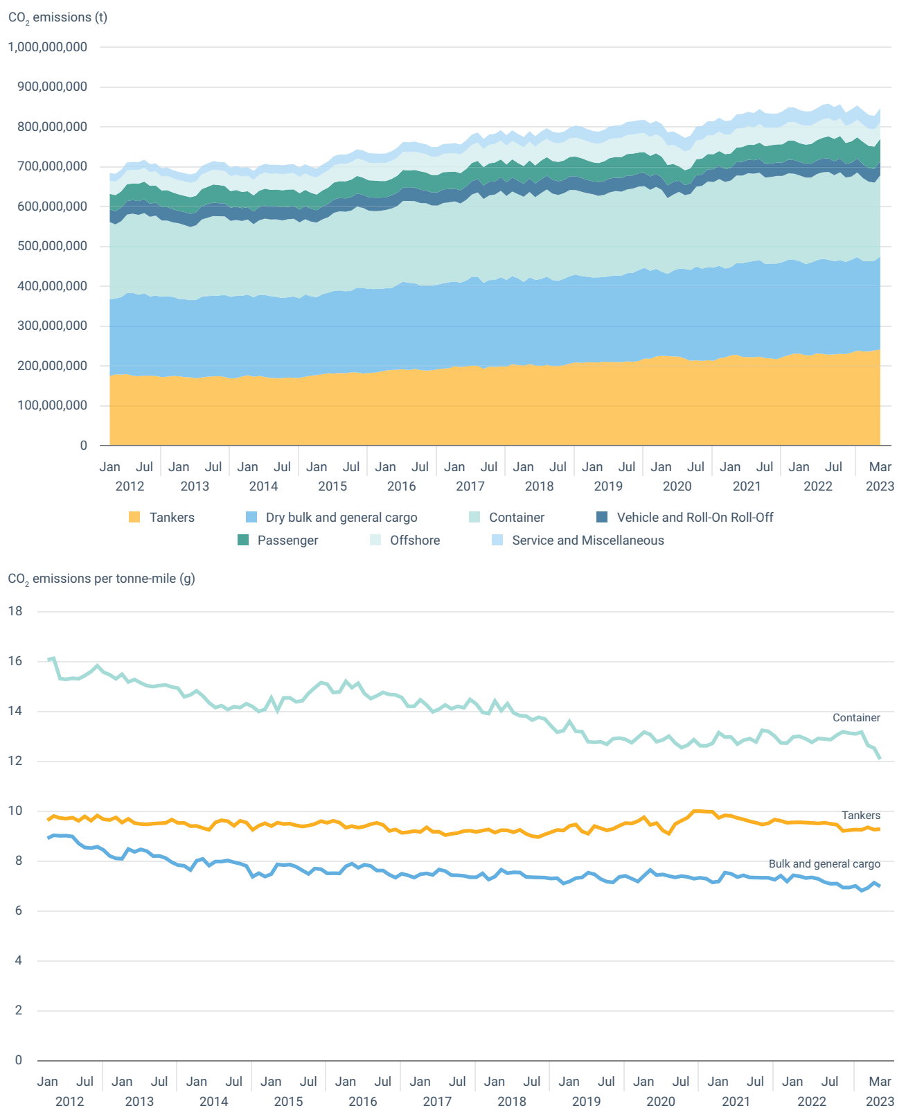
Figure 3.3 Total CO 2 emissions per ship type, 2012-2023 (above); CO 2 emissions per tonne-mile for world fleet monthly three main ship types, 2012-2023 (below)
