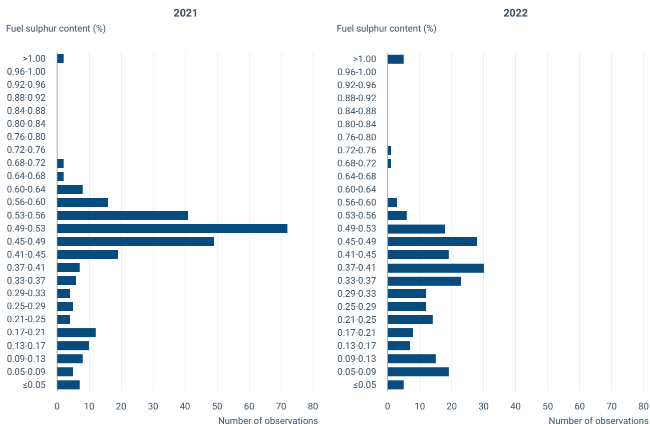
Figure 2.20 Distribution of sulphur emissions obtained through RPAS aerial measurements acquired outside SECA and port areas during 2021 (left) and 2022 (right)
