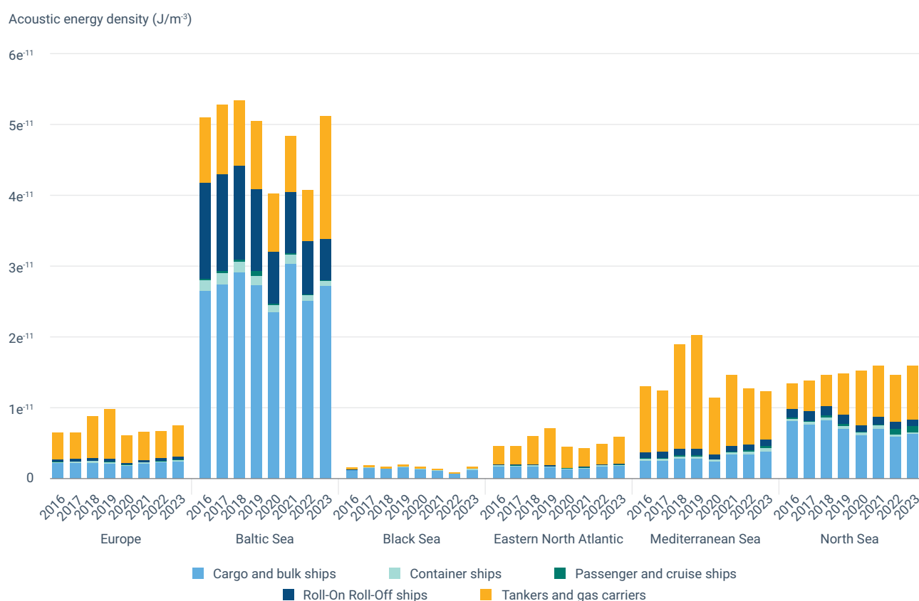
Figure 2.33 URN sound energy density at 63 Hz (Europe leftmost chart and regional seas) from 2016 to 2023
