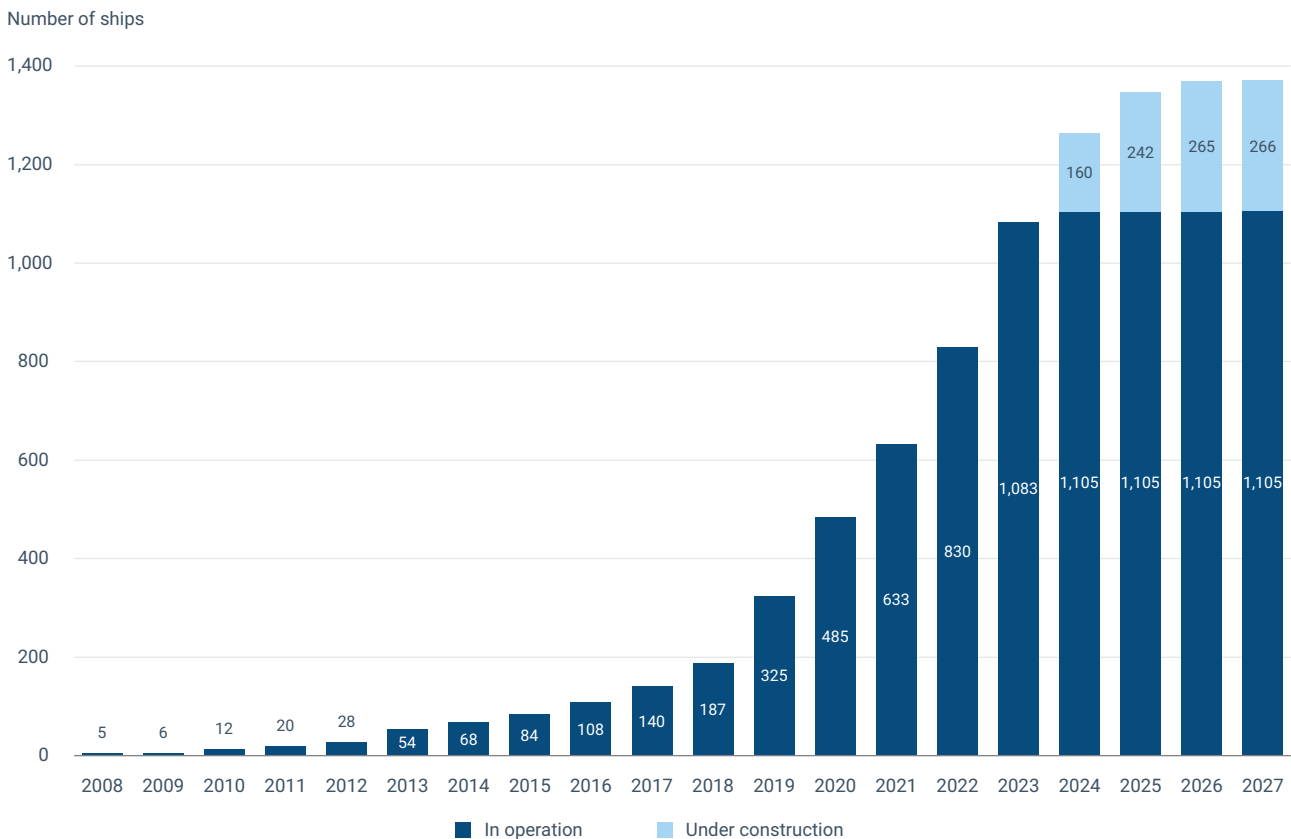
Figure 3.1 Total number of ships with batteries and known construction projects for 2024-2027
