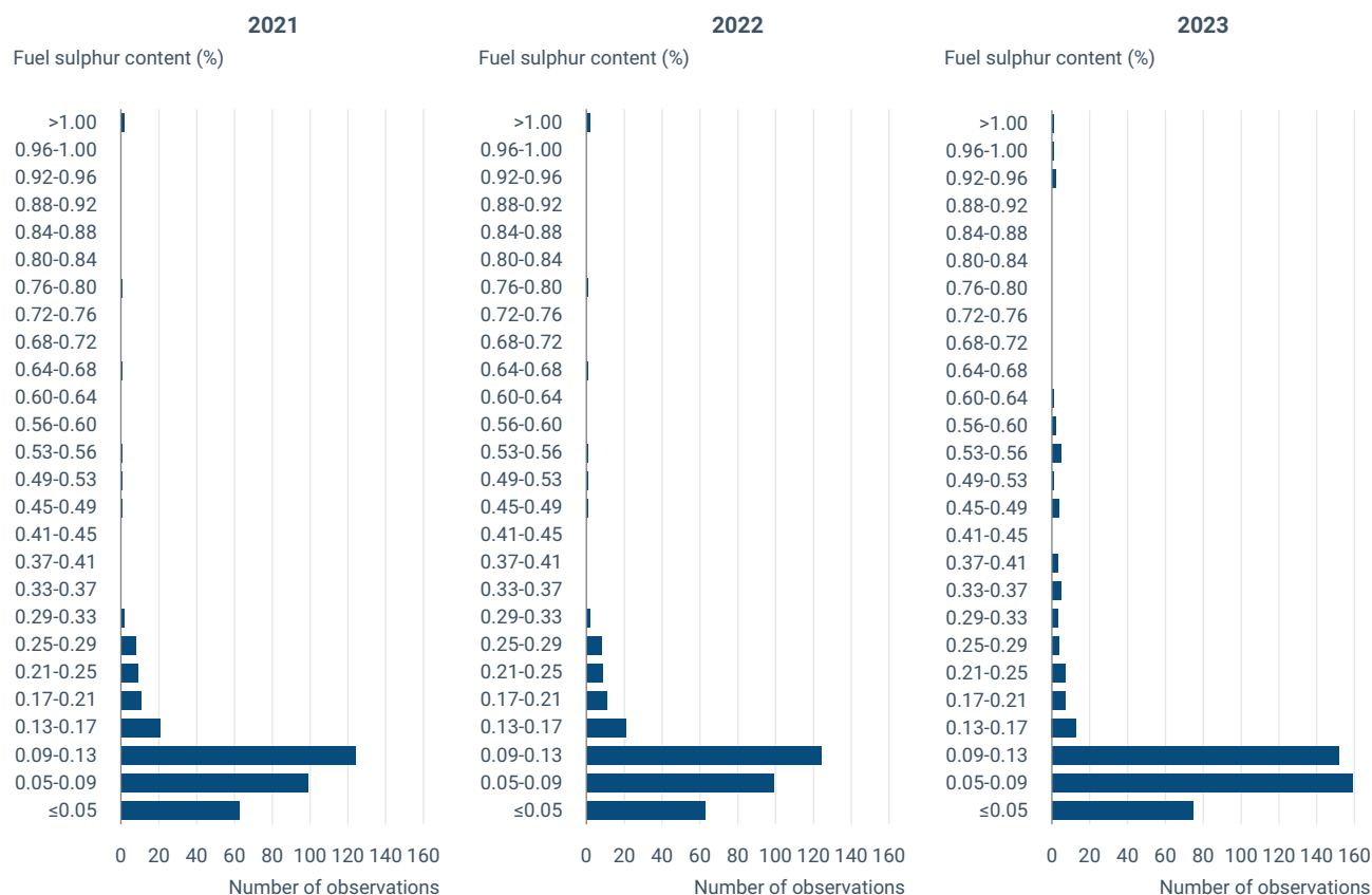
Figure 2.19 Distribution of sulphur emissions obtained through RPAS aerial measurements acquired in SECA and port areas during 2021 (left), 2022 (centre) and 2023 (right)
