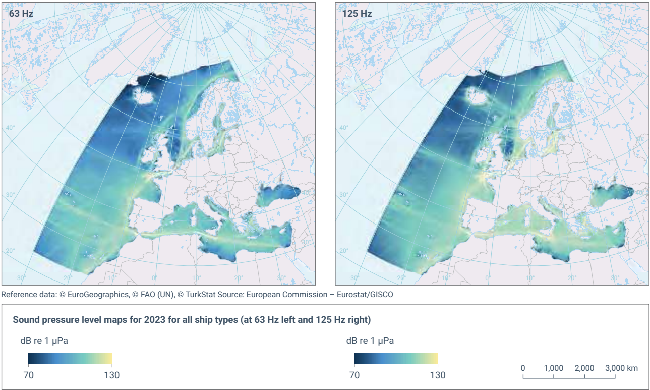
Map 2.7 Sound pressure level maps for 2023 for all ship types (at 63 Hz left and 125 Hz right)
