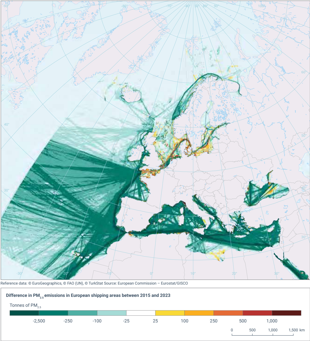
Map 2.6 Difference in PM 2.5 emissions in European shipping areas
