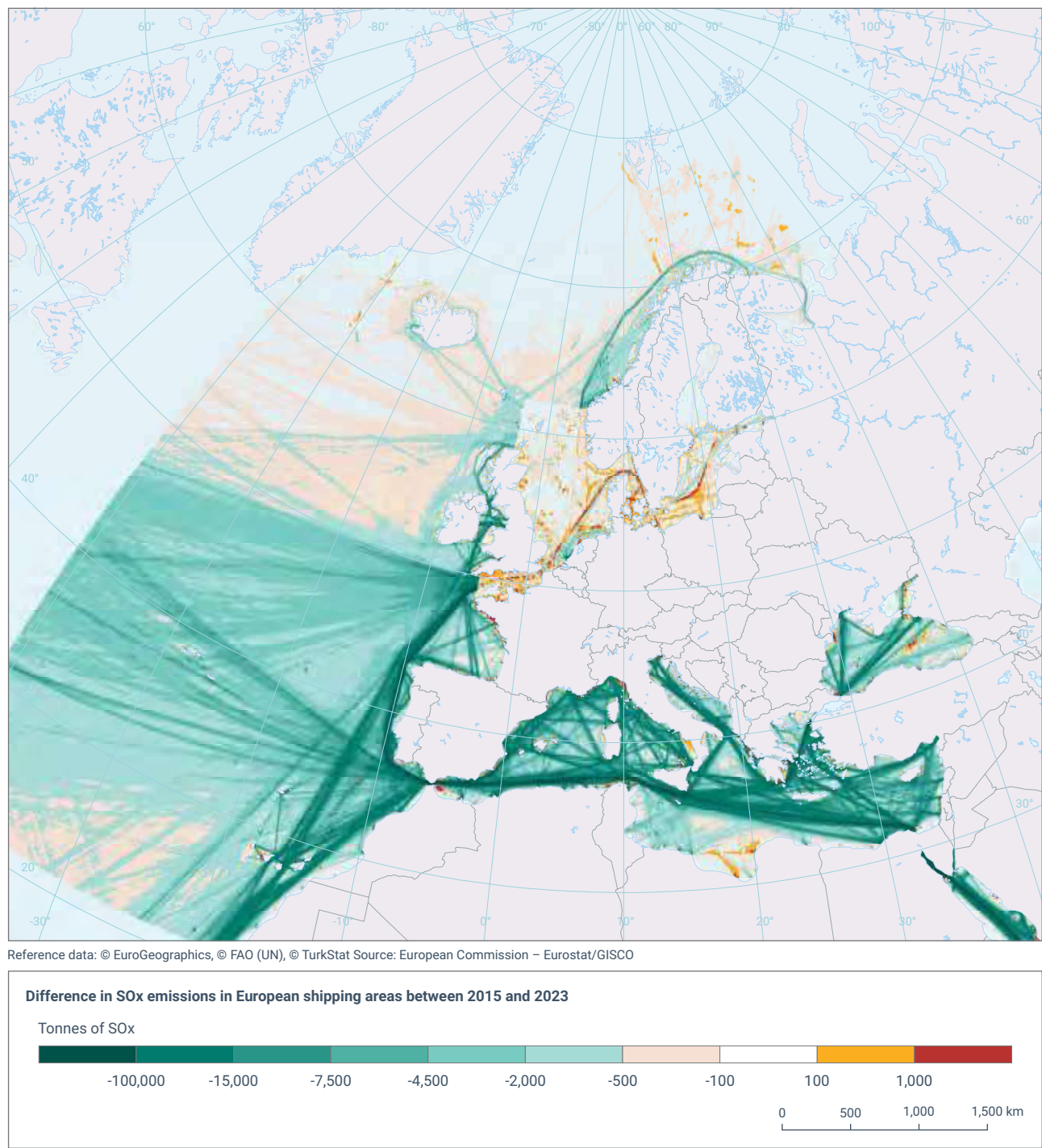
Map 2.4 Difference in SOx emissions across Europe's shipping areas
